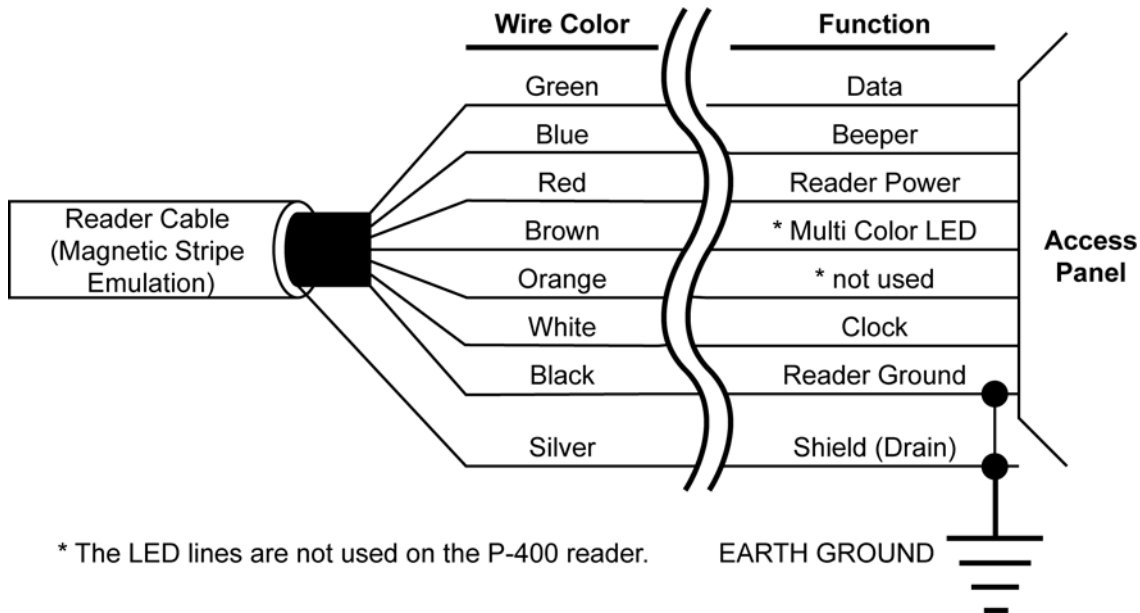
Figure 1: : Magnetic Stripe Format Wiring Connections
